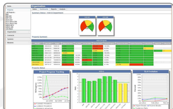
Data Warehouse
