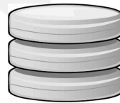
Data Warehouse
